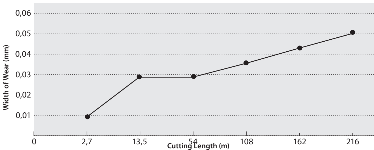
Wear Amount
