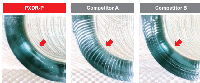
PXDR-P achieved fair finished surface with less chattering at the corner of work versus the competition.
